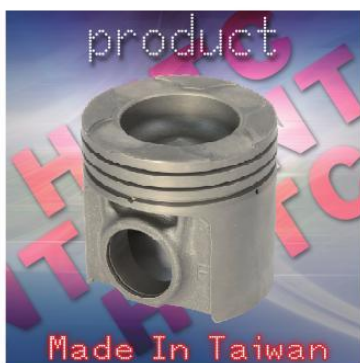
ENGINE PISTON: CASTING IRON 引擎活塞D125*D75*H117*R3 S6D125 / PC300-3 / PC400-3 / PC400-5 / PC400-6 6152-31-2113-Y
