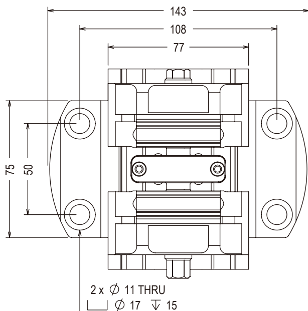
3" Installation Diagram
