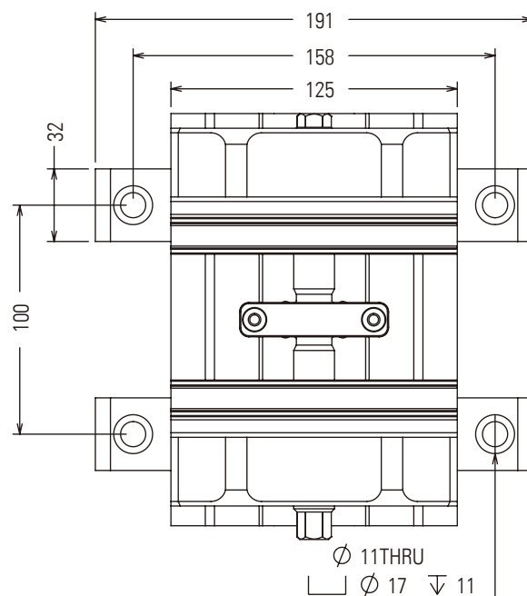
5" Installation Diagram
